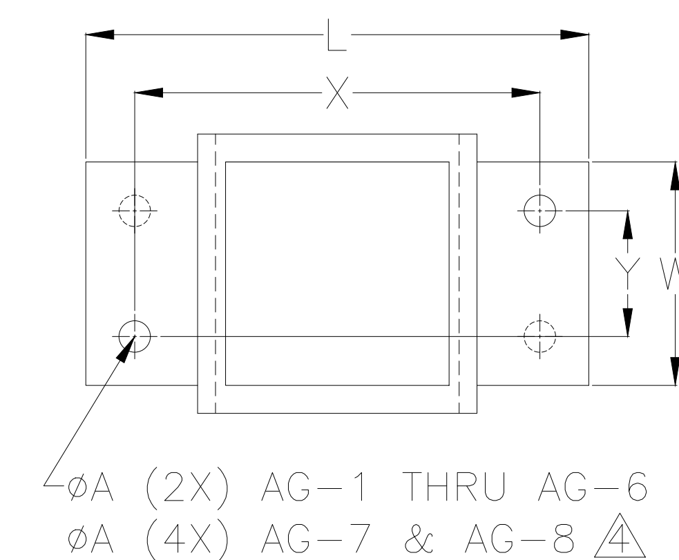
ANCHORING PLAN
